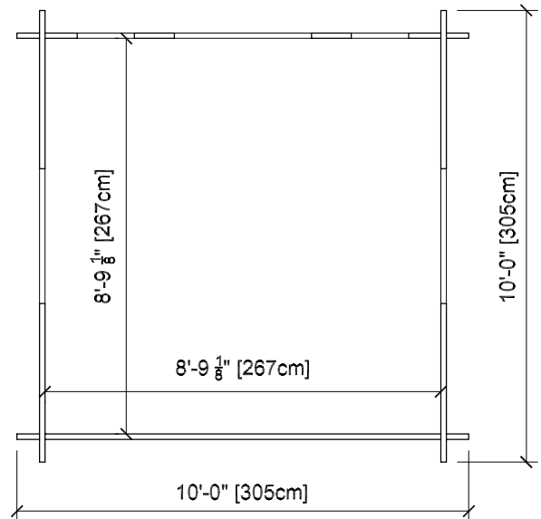
Floor Plan
